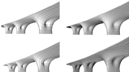
Figure 13: Explorations into subdividing the mold in flat or singly curved panels.
