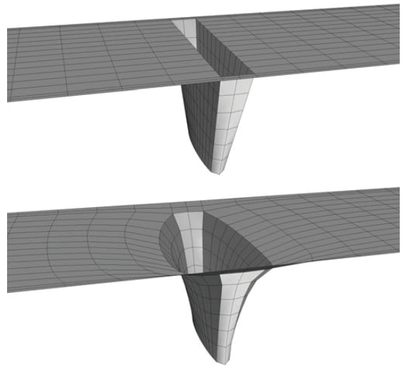
Figure 10: The modified / tailored mesh before and after relaxation.
