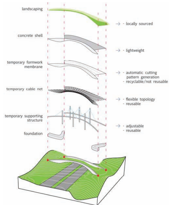
Figure 6: Exploded view of the construction elements
