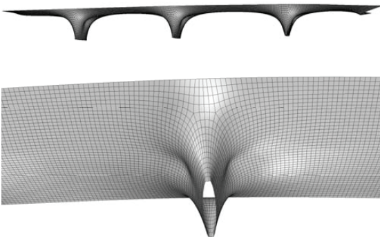
Figure 12: The final mesh
