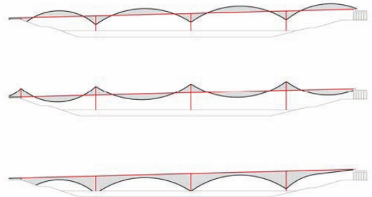
Figure 8: The overall shape of the bridge is derived by rotation and translation of the bending moment diagram
