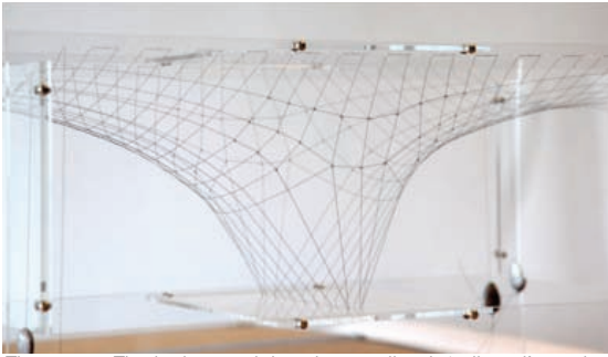
Figure 11: Final wire model of the modified, 'tailored' mesh.
