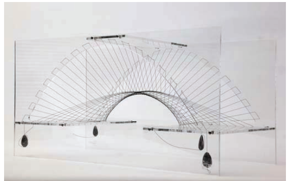
Figure 4: Final wire model of the cable net
