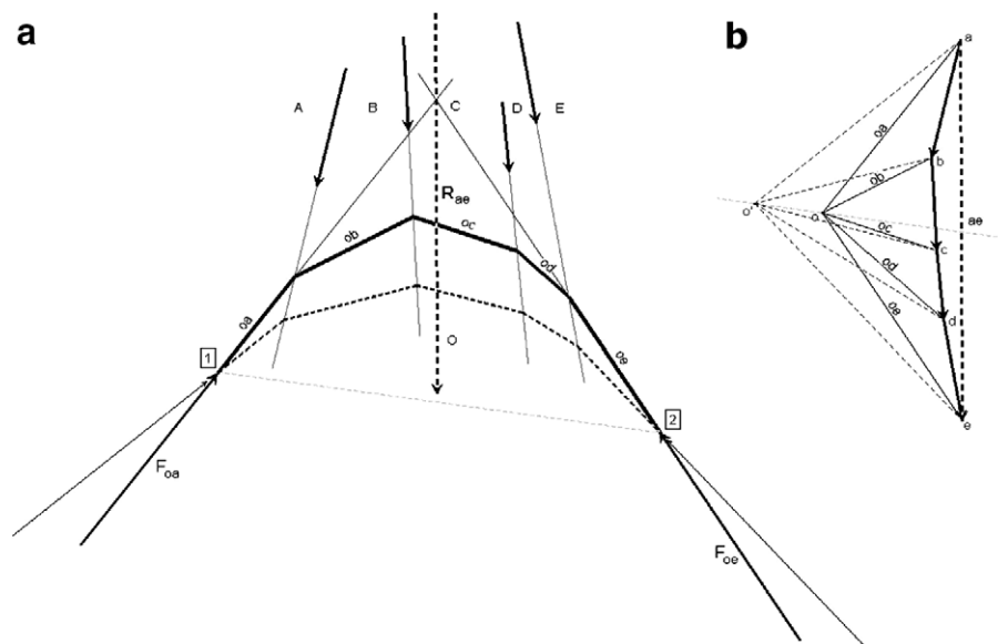
Fig. 2. Graphic statics allows the construction of (a) funicular shapes (only tension or compression) for a given set of loads using Bow's notation and (b) the corresponding force polygons that give the magnitude of the forces of the segments in the funicular polygon [19].
