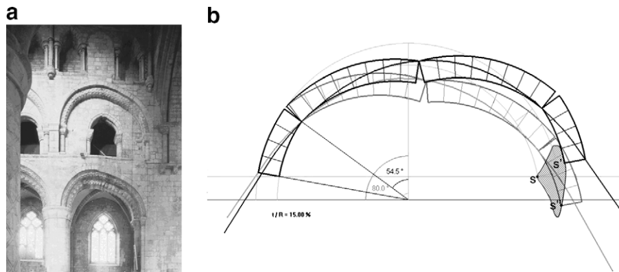
Fig. 10. (a) Example of highly deformed arches in Selby Abbey, England, and (b) two limit states of an arch. The arch in position s is in its undeformed state. (Photo source: Jacques Heyman).
